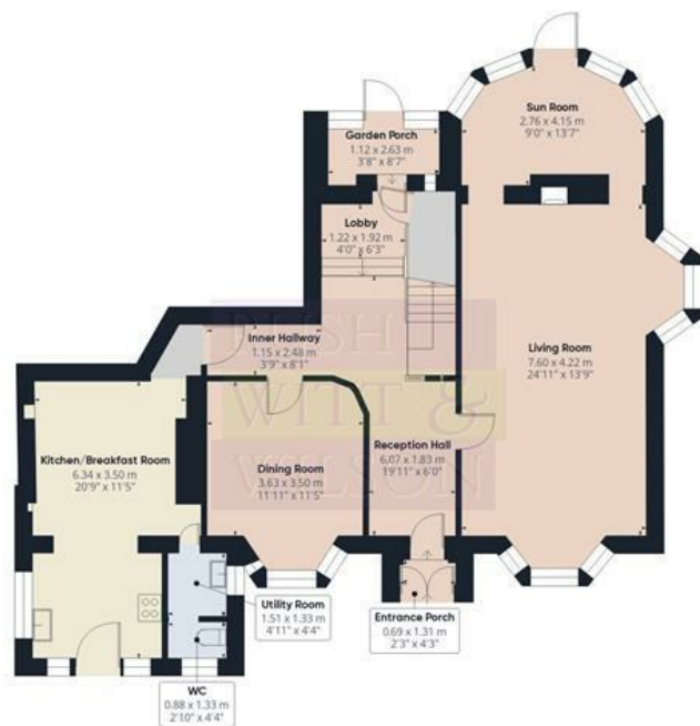
Floor 0 Building 1
